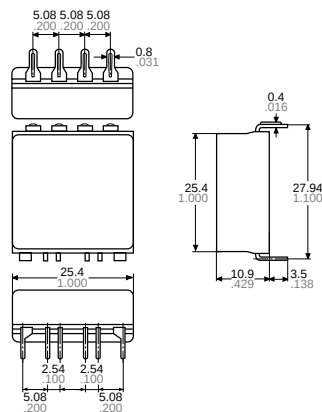
External dimensions
