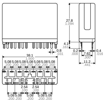
External dimensions
