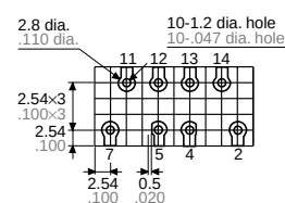
PC board pattern (Bottom view)
