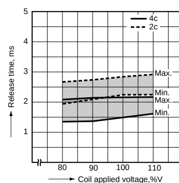
4. Release time (single side stable)
