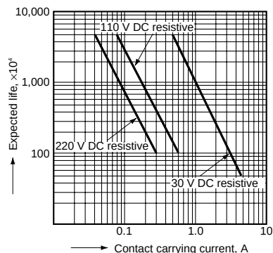
1.-(1) Life curve (2 Form C, 4 Form C)
