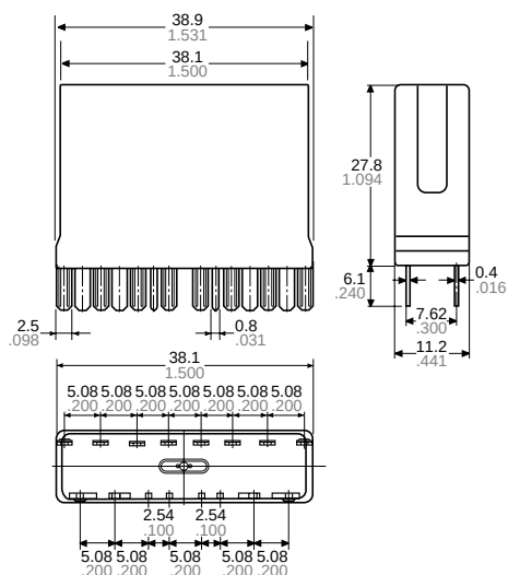
External dimensions
