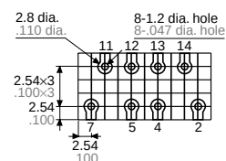
PC board pattern (Bottom view) Single side stable
