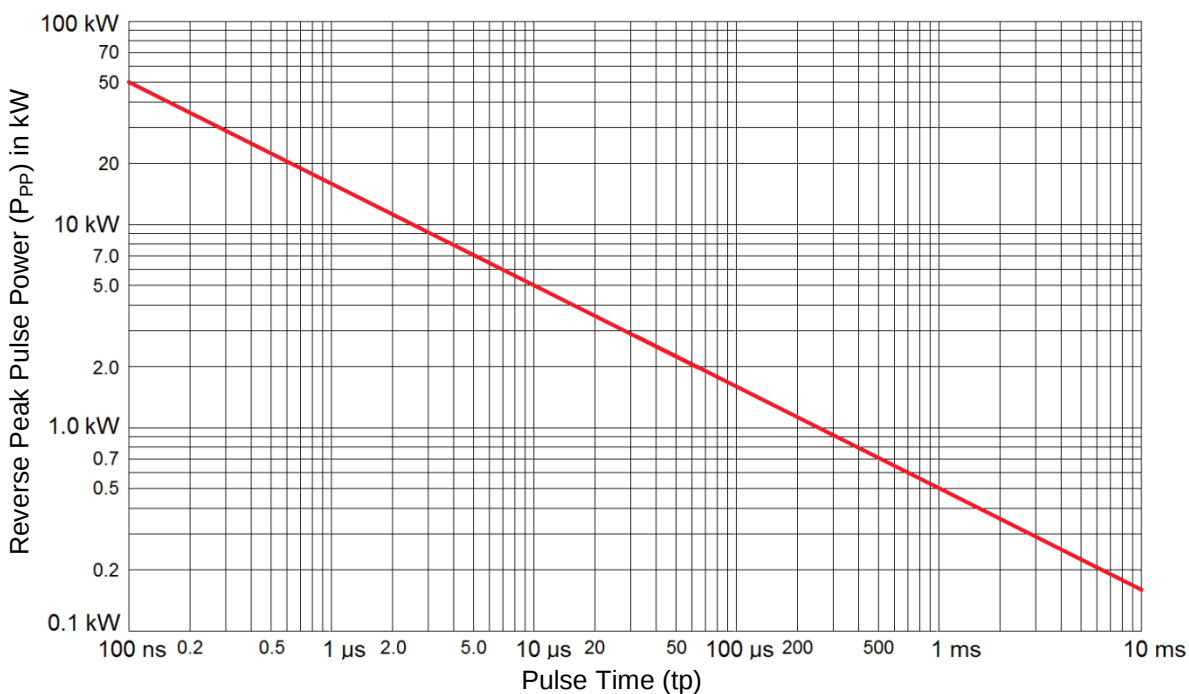
FIGURE 1 Peak Pulse Power vs Pulse Time
