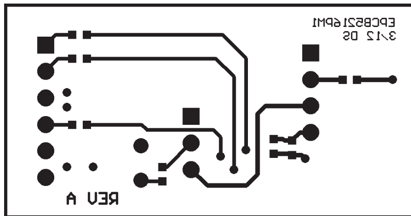
Figure 6. MAX5216PMB1 Peripheral Module PCB Layout—Solder Side
