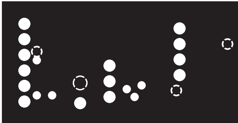
Figure 5. MAX5216PMB1 Peripheral Module PCB Layout—Inner Layer 2 (Power)
