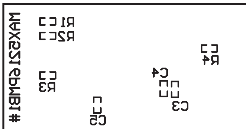
Figure 7. MAX5216PMB1 Peripheral Module Component Placement Guide—Solder Side
