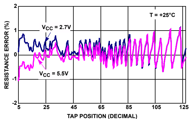
FIGURE 2. RESISTANCE ERROR vs TAP POSITION [ I(RW) = V_{CC}/R_{TOTAL} ] FOR 10kΩ (W)
