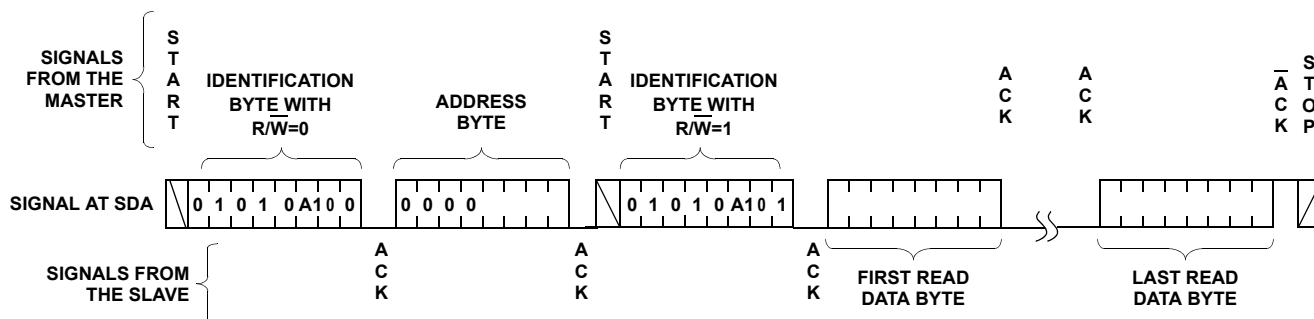
FIGURE 24. READ SEQUENCE
