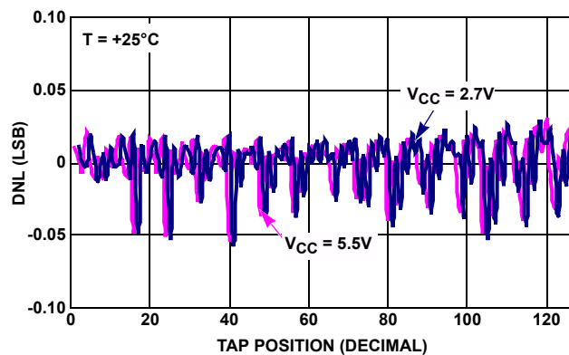
FIGURE 12. DNL vs TAP POSITION IN VOLTAGE DIVIDER MODE FOR 10kΩ (W)
