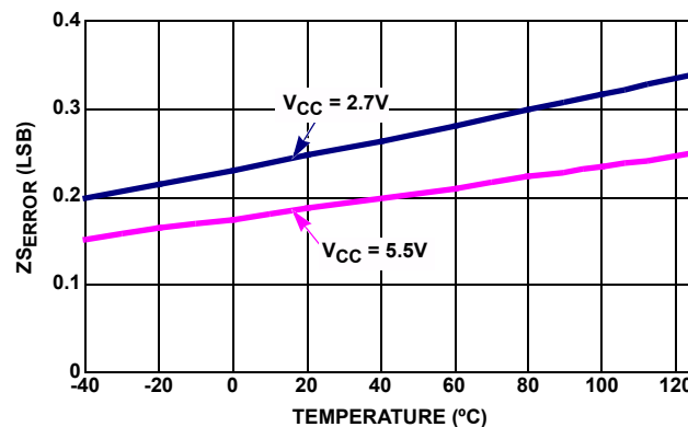
FIGURE 14. ZSEERROR vs TEMPERATURE FOR 10kΩ (W)
