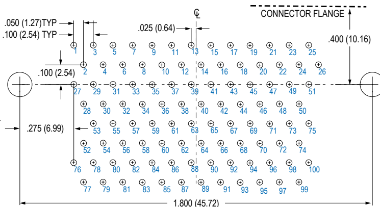
100 PIN M83513/12-H
