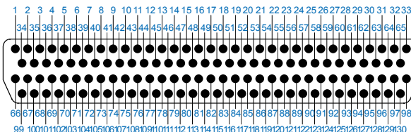
130 pin
