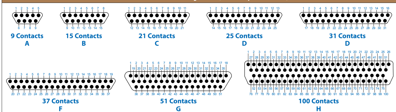
MIL-DTL-83513 contact arrangements (face view pin connector)
