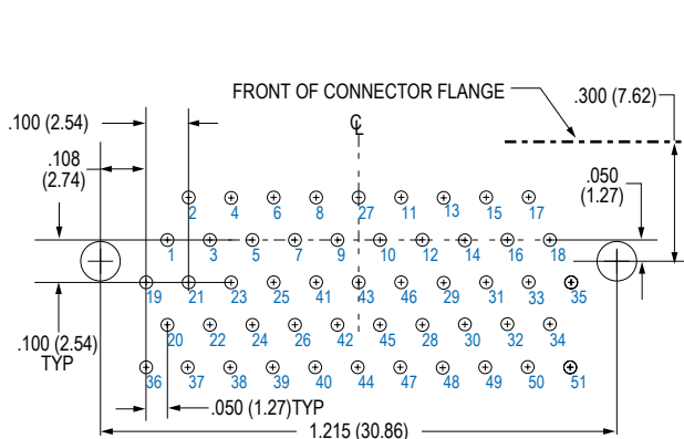
51 PIN M83513/11-G
