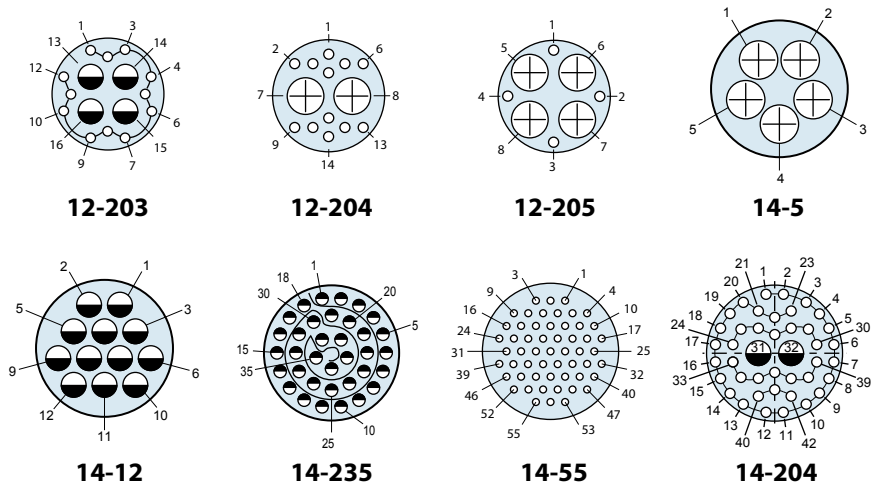
Mating Face View of Pin Connector (socket connector numbers are reversed)
