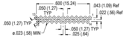
25 Socket
