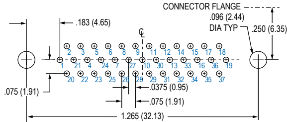
37 PIN
