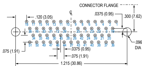
51 SOCKET
