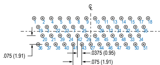
51 PIN
