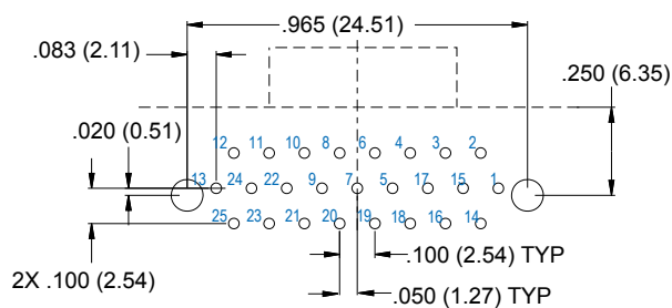
25 Socket
