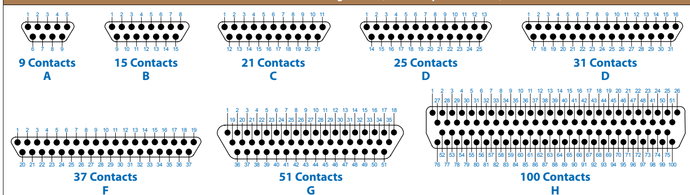
MIL-DTL-83513 contact arrangements (face view pin connector)
