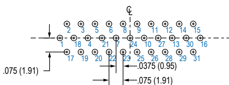
31 PIN
