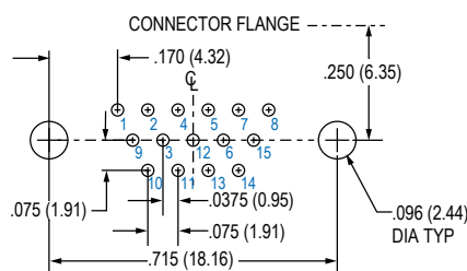
15 PIN
