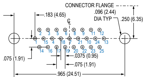
25 PIN
