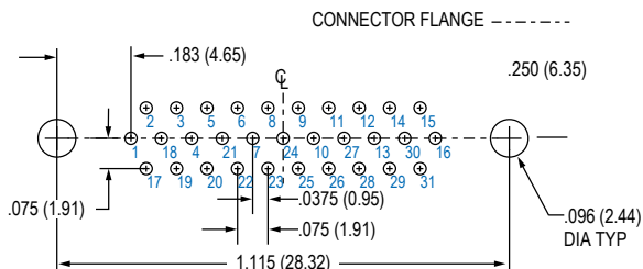
31 PIN
