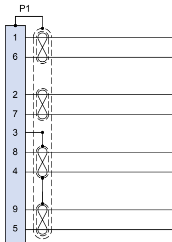
Single Ended Wiring Diagram (P)
