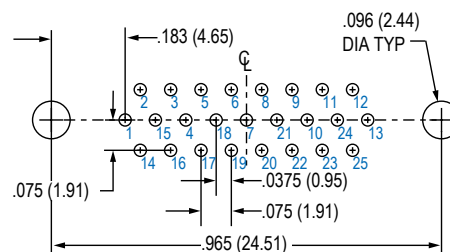
25 PIN
