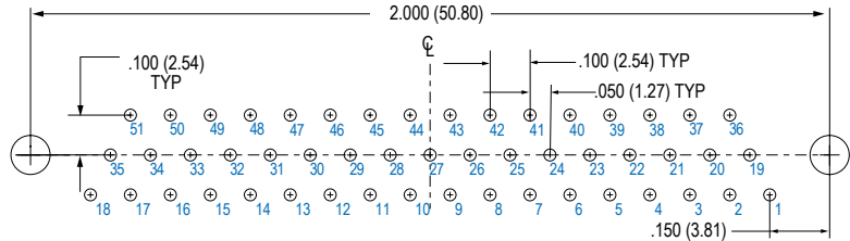
51 PIN
