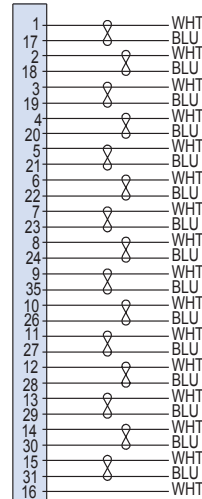
31 Contacts
