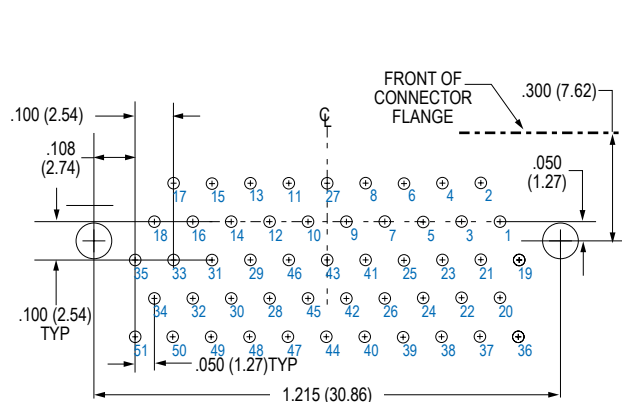
51 SOCKET M83513/14-G
