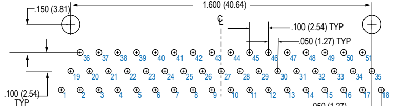
51 SOCKET
