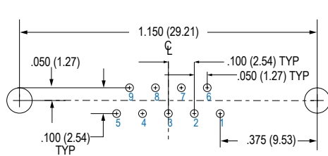
9 PIN
