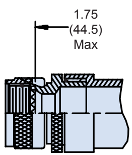
STYLE 2 STRAIGHT
