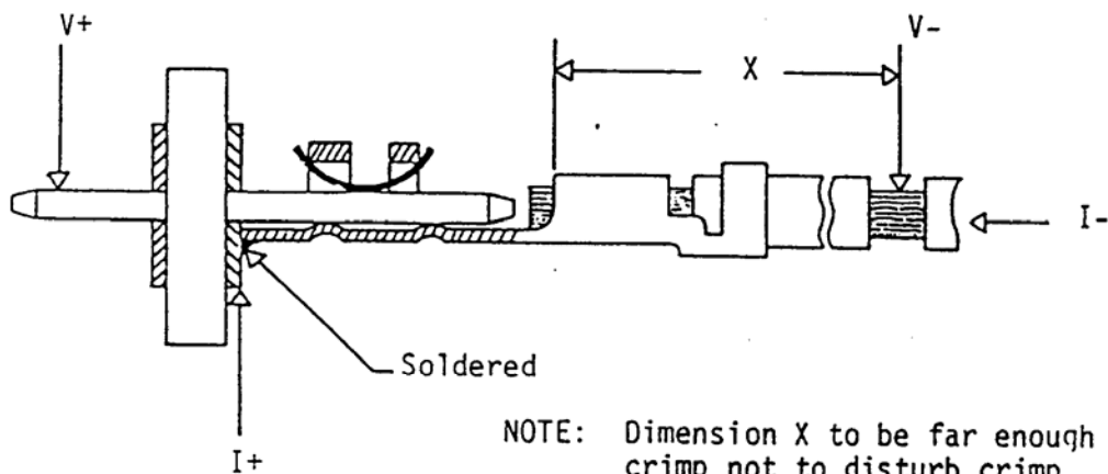
FIGURE 3 CONTACT RESISTANCE
