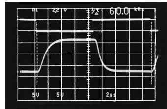
Transmitter Output R L = 3kΩ, C L = 2,500pF
