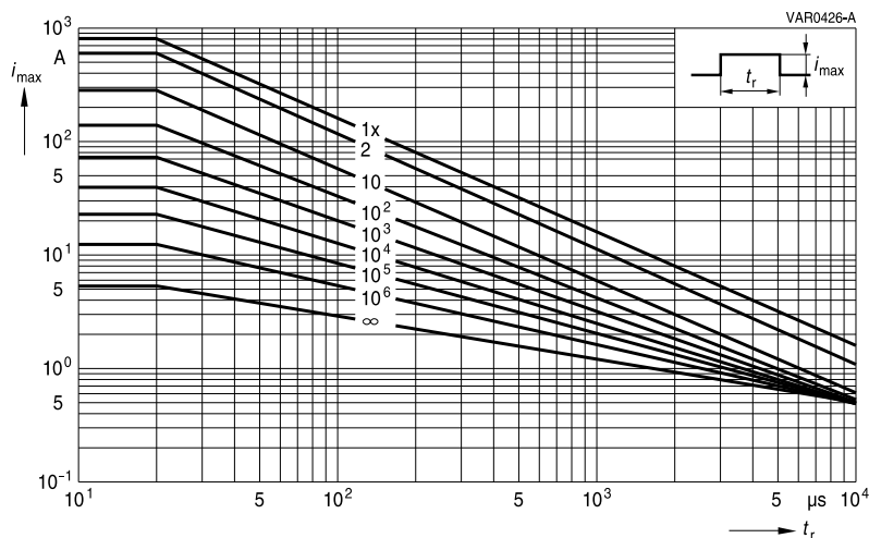
SIOV-S05K130 ... K300E2
