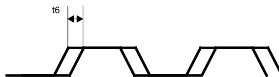
Figure 10. Peak-to-Peak Jitter
