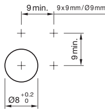
Mounting cut-outs [mm]
