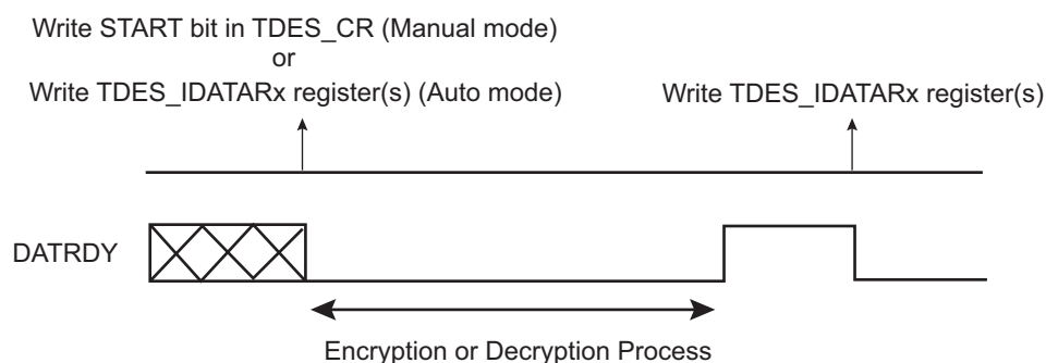
Figure 59-2. Manual and Auto Modes with LOD = 1
