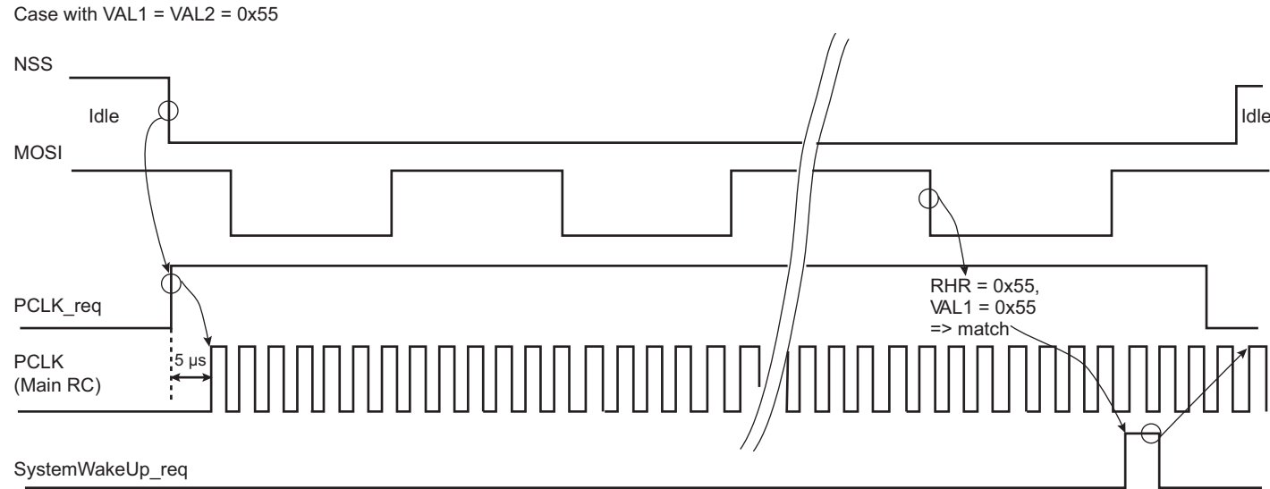
Figure 46-14. Asynchronous Wakeup Use Case Example
