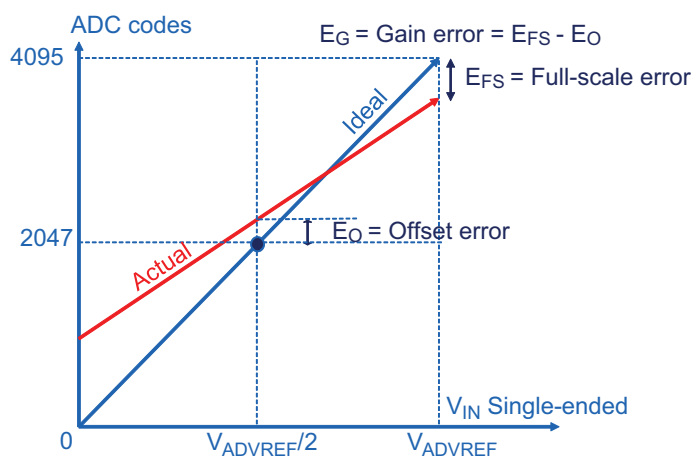
Figure 62-6. Gain and Offset Errors in Single-ended Mode
