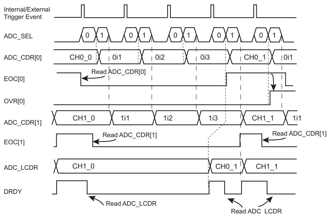
Figure 61-11. Digital Averaging Function Waveforms Over Multiple Trigger Events
