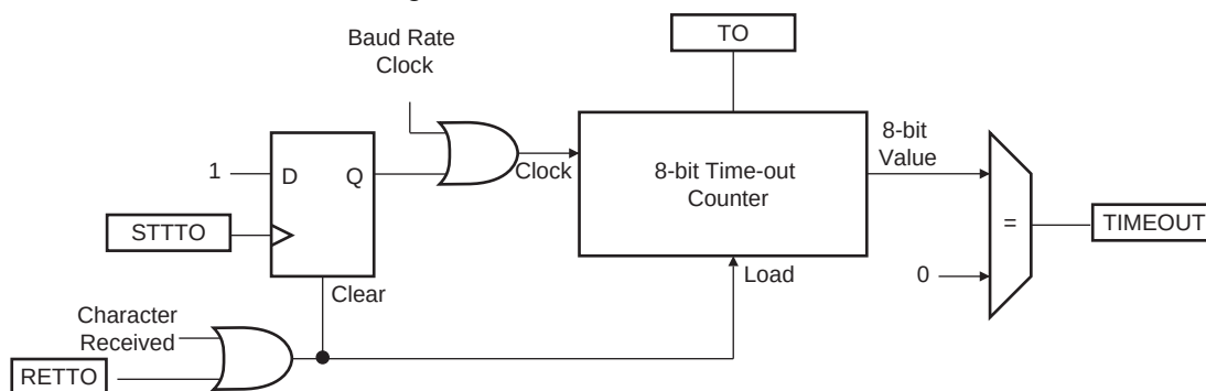
Figure 45-10. Receiver Timeout Block Diagram
