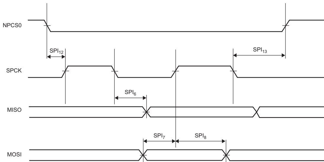
Figure 62-21. FLEXCOM in SPI Slave Modes 0 and 3
