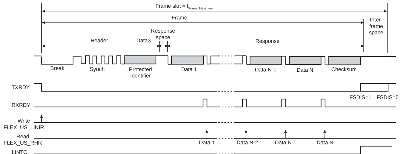
Figure 44-48. Master Node Configuration, NACT = SUBSCRIBE
