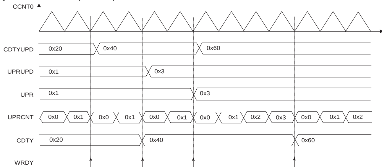
Figure 53-20. Method 2 (UPDM = 1)
