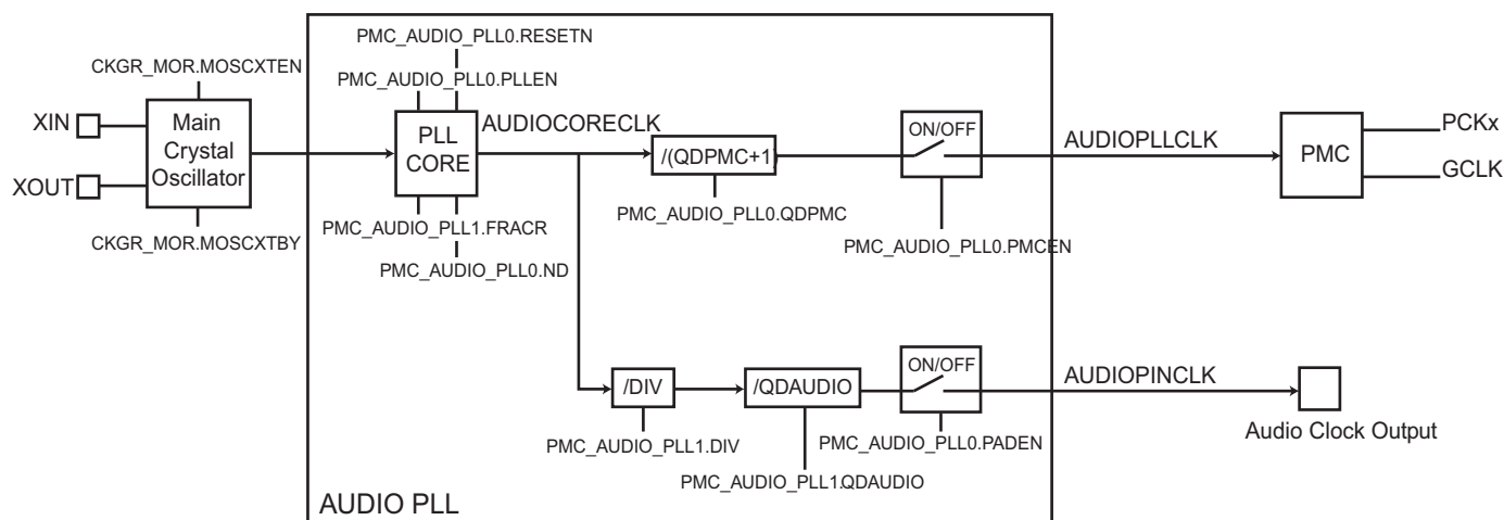
Figure 29-7. Audio PLL
