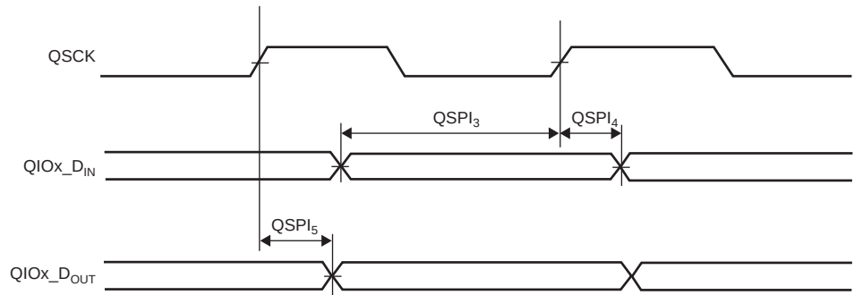
Figure 62-26. QSPI Master Mode 1
