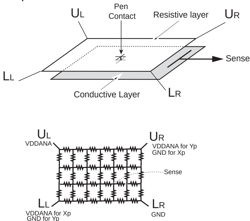
Figure 61-17. 5-Wire Principle
