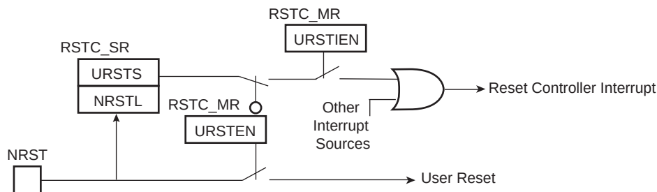
Figure 22-2. NRST Manager
