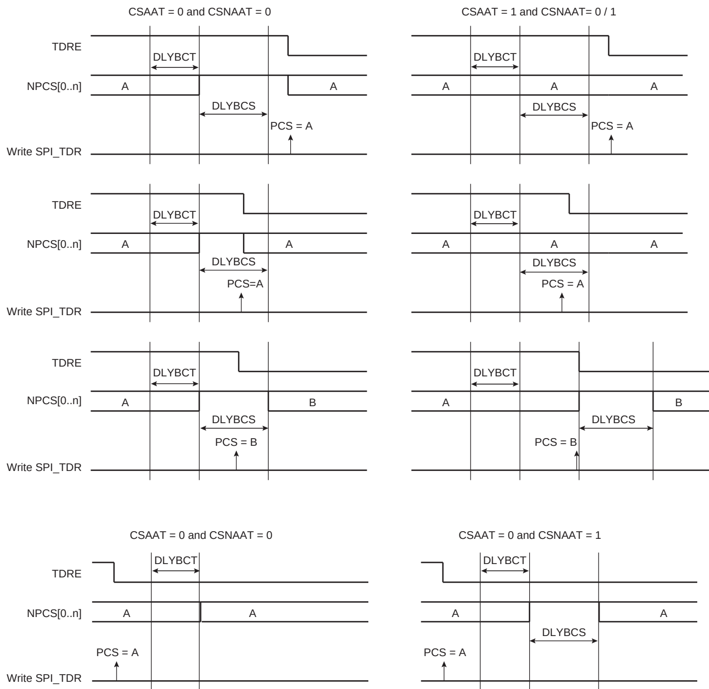
Figure 46-11. Peripheral Deselection
