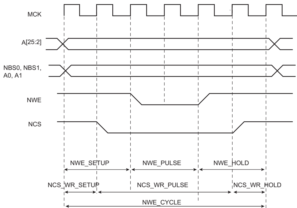
Figure 34-10. Write Cycle
