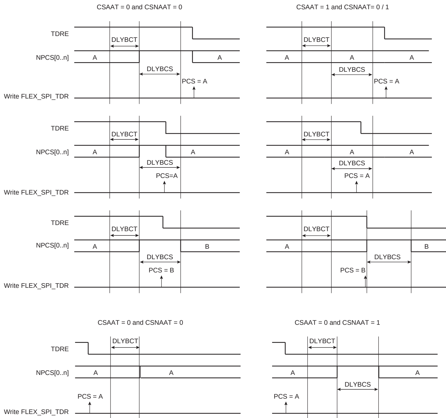
Figure 44-73. Peripheral Deselection
