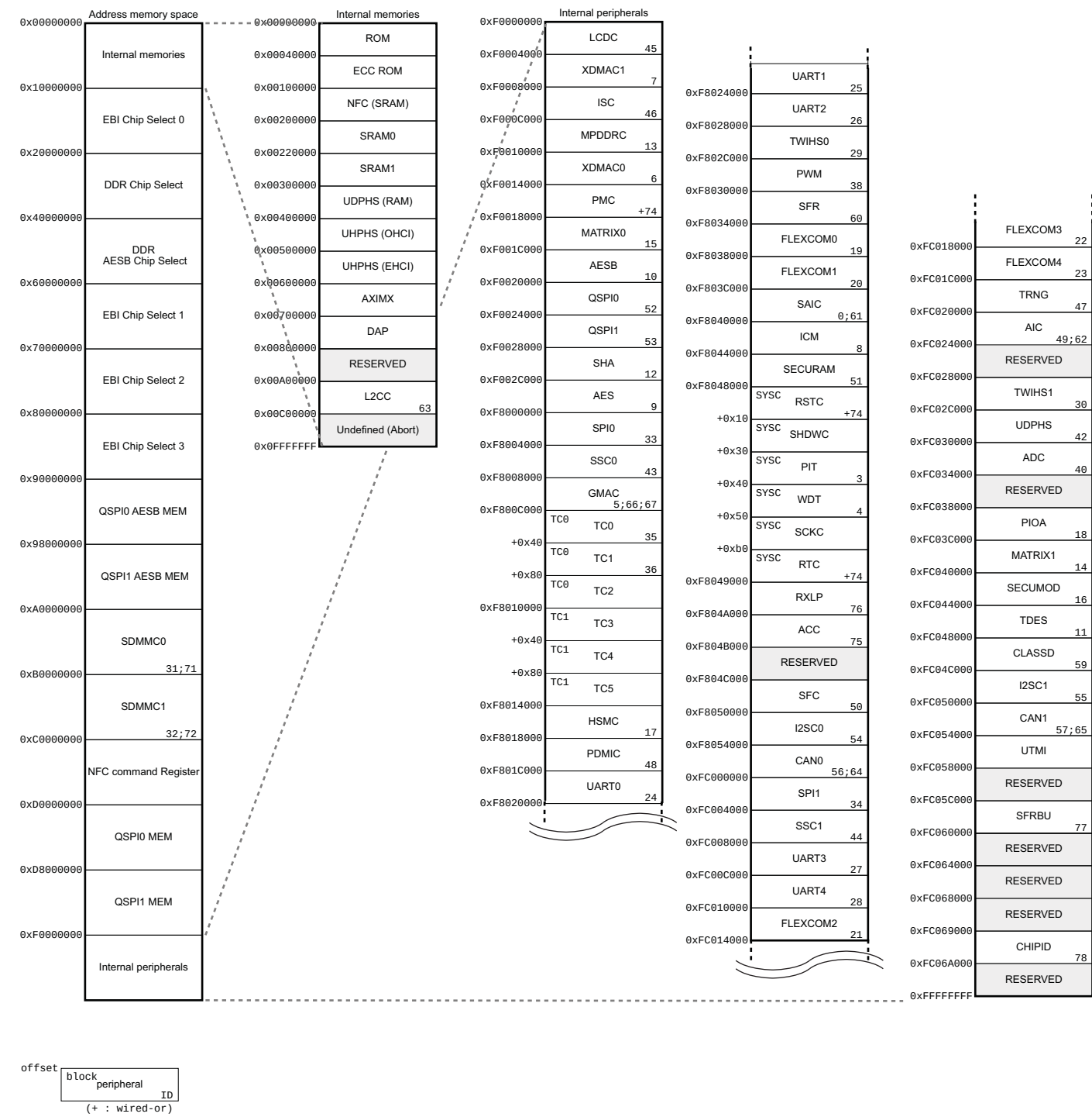
Figure 7-1. Memory Mapping
