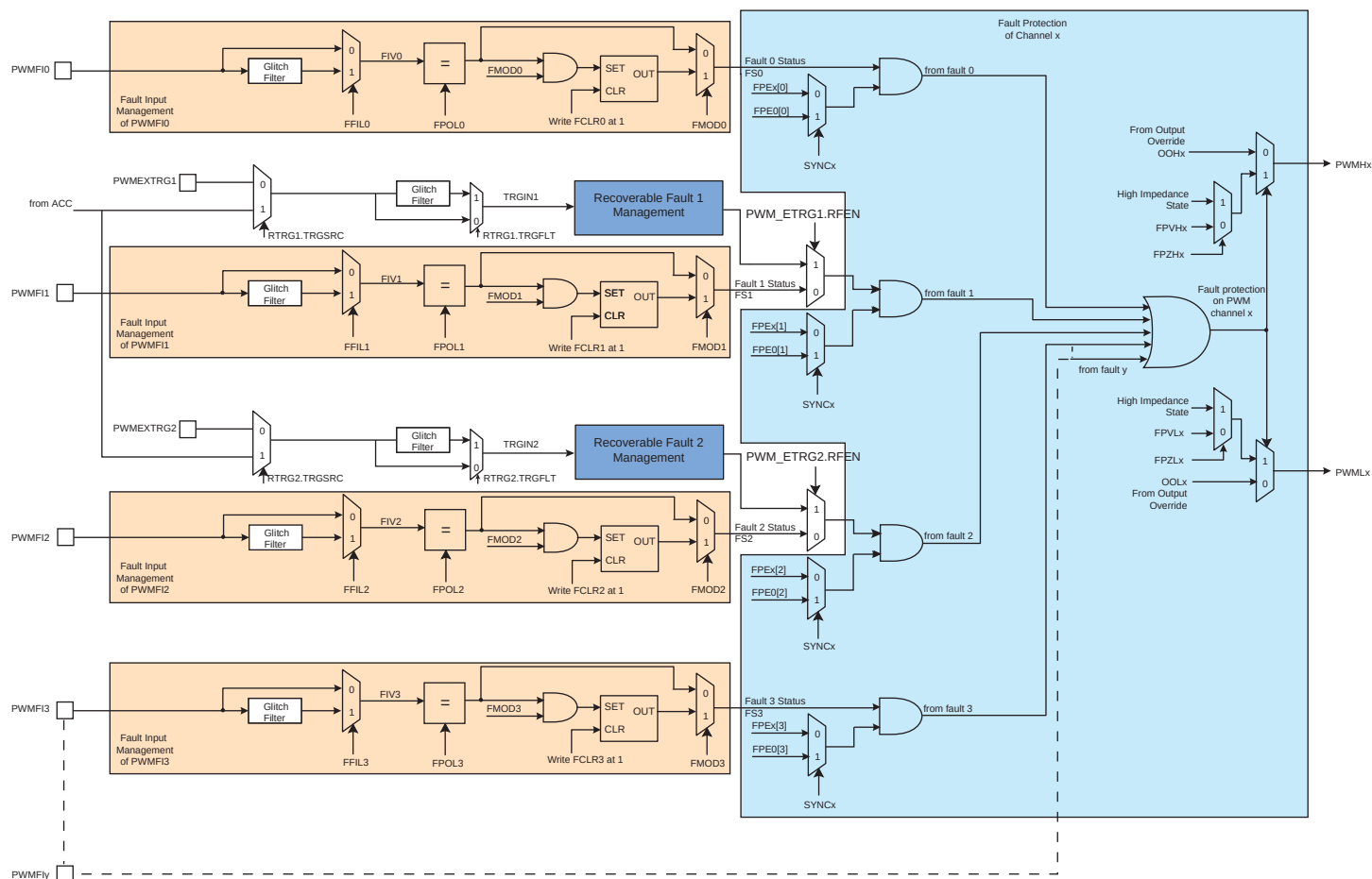
Figure 53-16. Fault Protection
