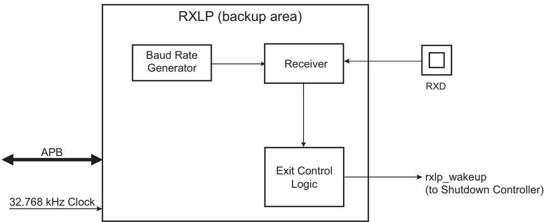
Figure 27-1. RXLP Functional Block Diagram
