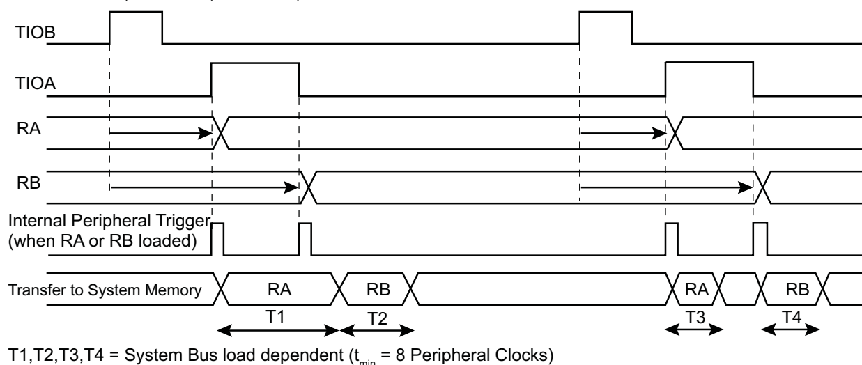
Figure 51-5. Example of Transfer with DMAC in Capture Mode
