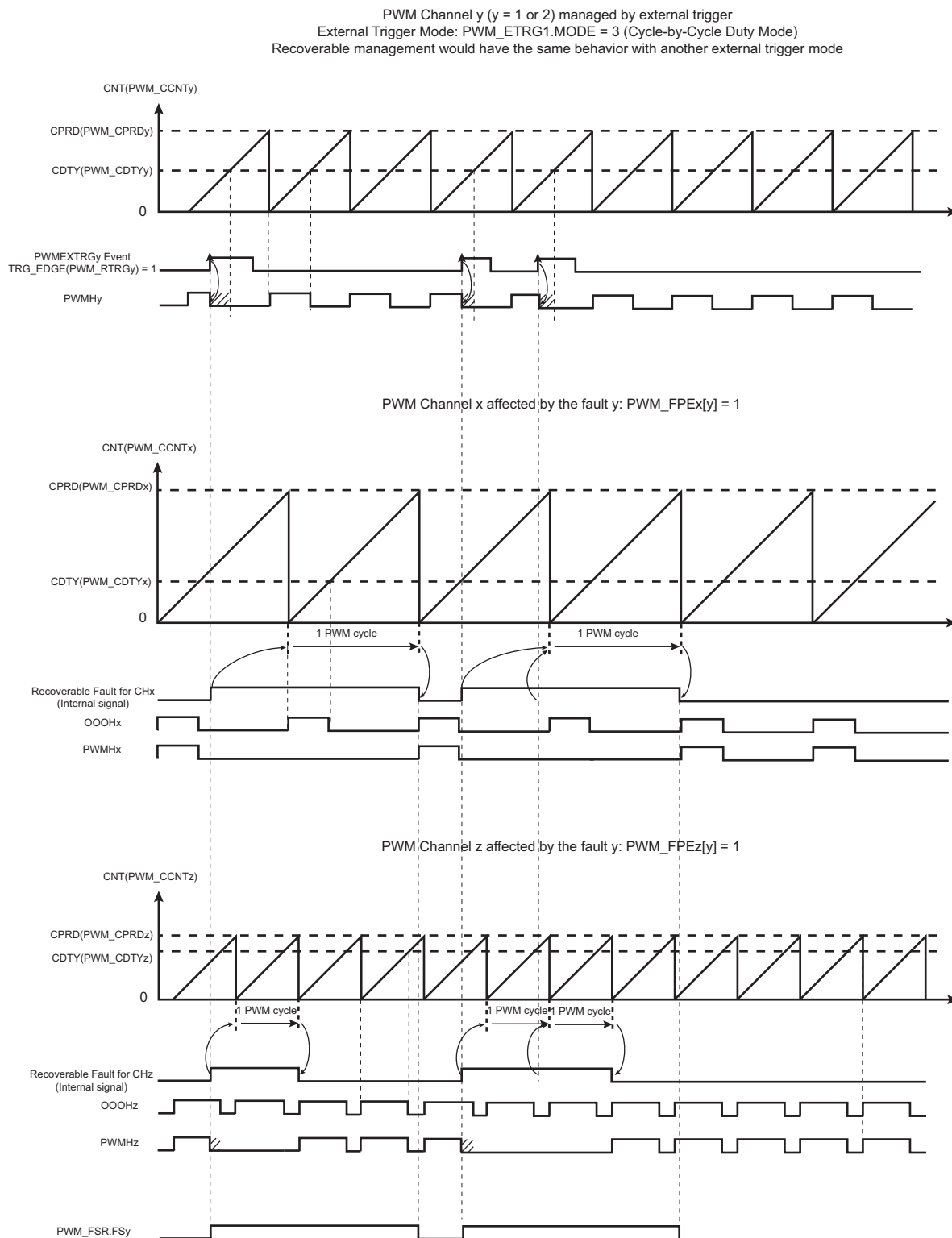
Figure 53-17. Recoverable Fault Management
