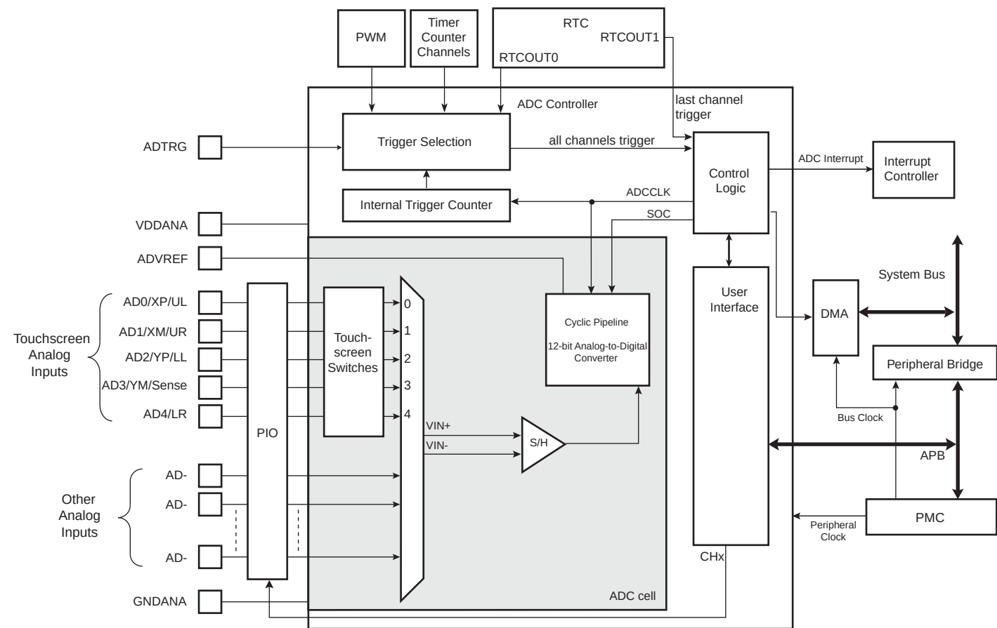
Figure 61-1. Analog-to-Digital Converter Block Diagram
