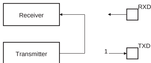
Figure 44-58. Local Loopback Mode Configuration
