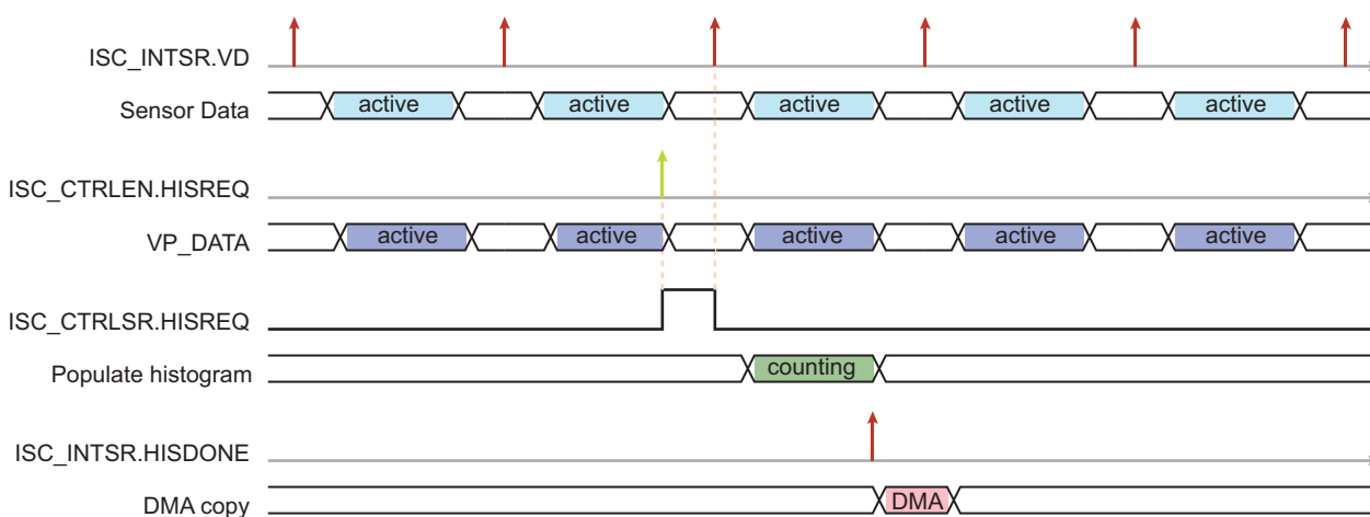
Figure 49-36. Histogram Request timing diagram
