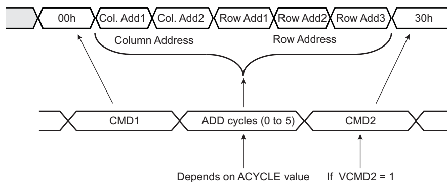
Figure 34-31. NFC/NAND Flash Access Example
