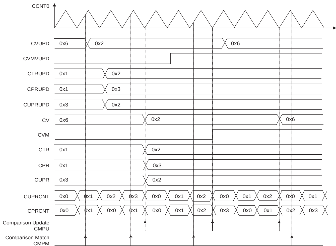
Figure 53-24. Comparison Waveform
