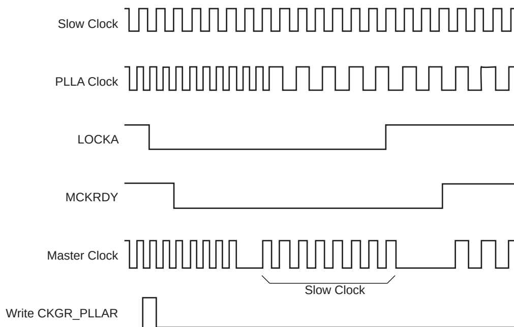
Figure 30-14. Change PLLA Programming
