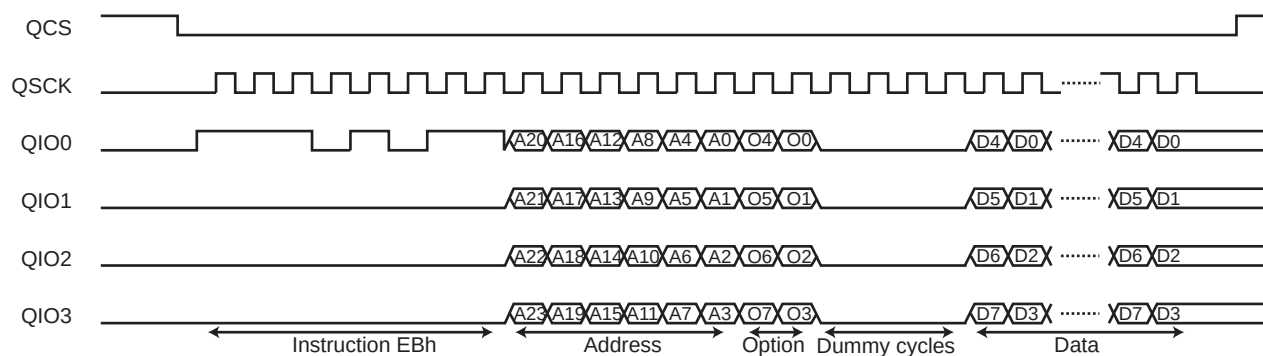
Figure 47-8. Instruction Frame
