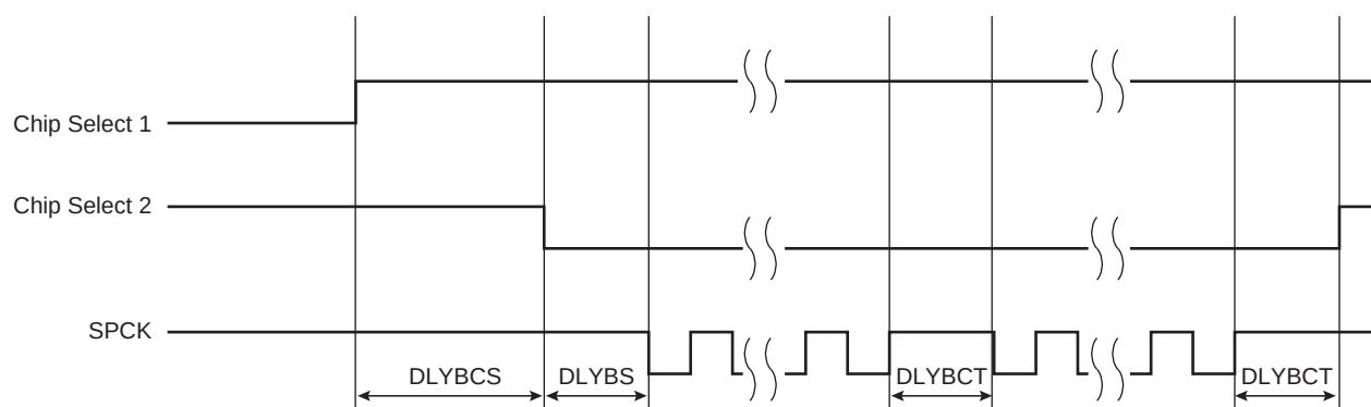
Figure 46-9. Programmable Delays
