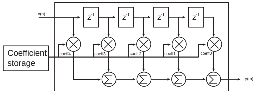
Figure 36-7. Horizontal Resampler Filter Architecture
