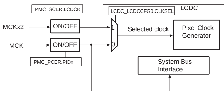
Figure 30-4. LCDCLK Clock Configuration
