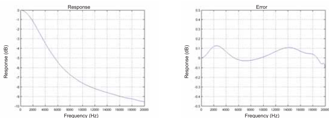
Figure 40-9. De-emphasis Filter: Frequency Response & Error ( f_s = 44.1 kHz)
