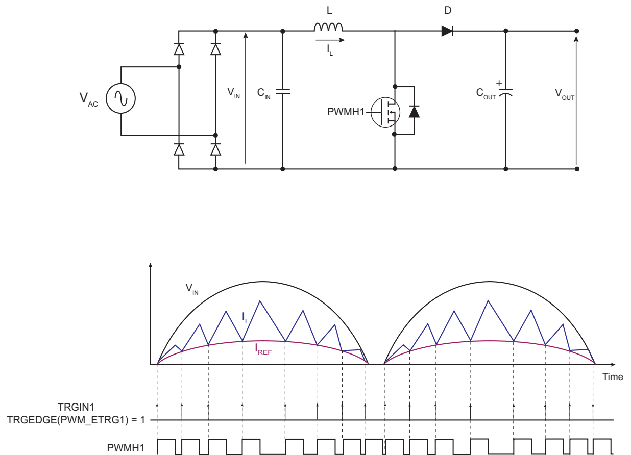
Figure 53-28. External PWM Reset Mode: Power Factor Correction Application
