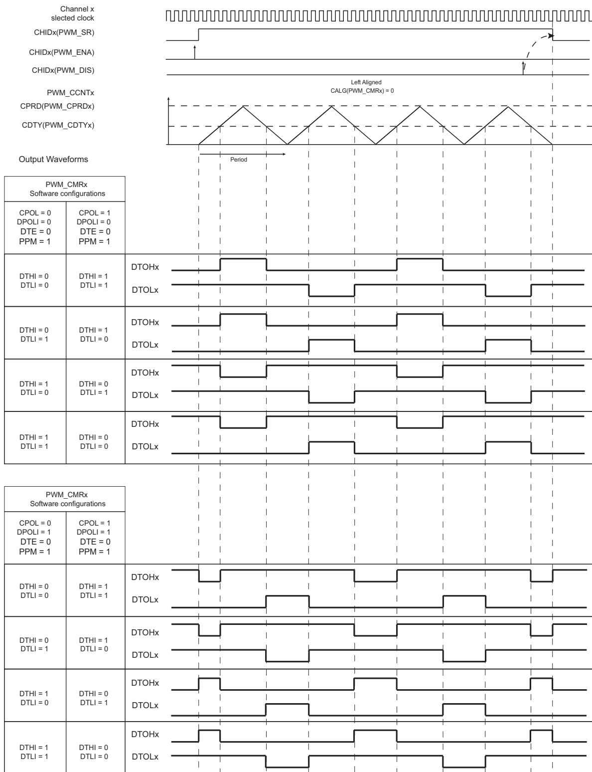
Figure 53-12. PWM Push-Pull Waveforms: Center-Aligned Mode
