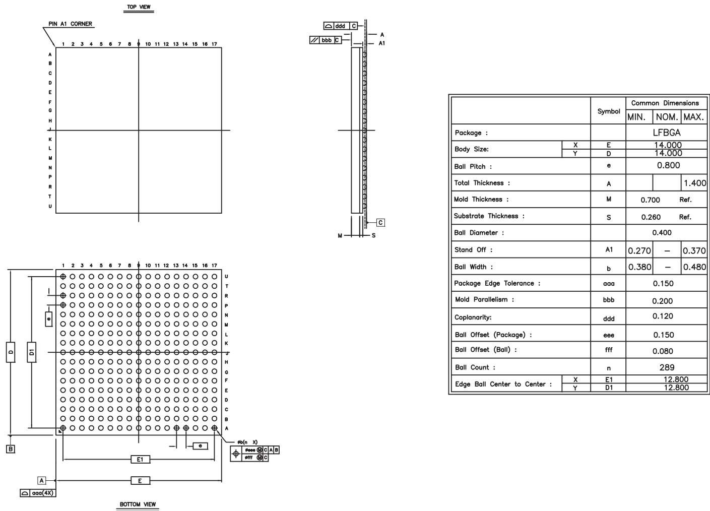
Figure 63-1. 289-ball LFBGA Package Drawing
