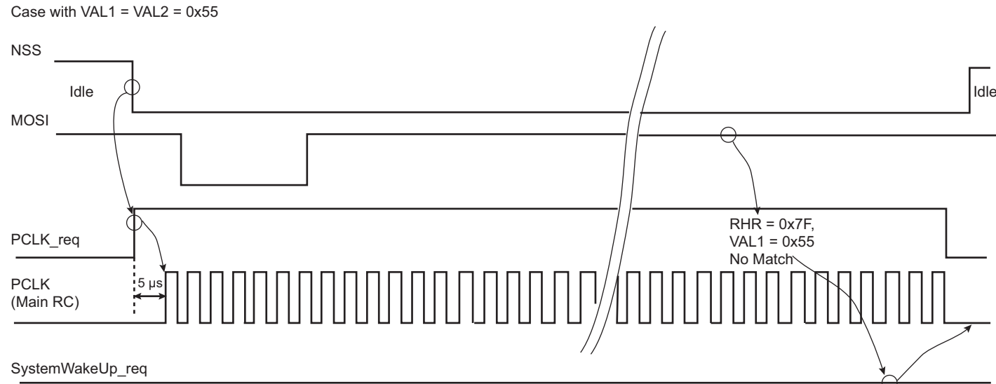
Figure 46-15. Asynchronous Event Generating Only Partial Wakeup
