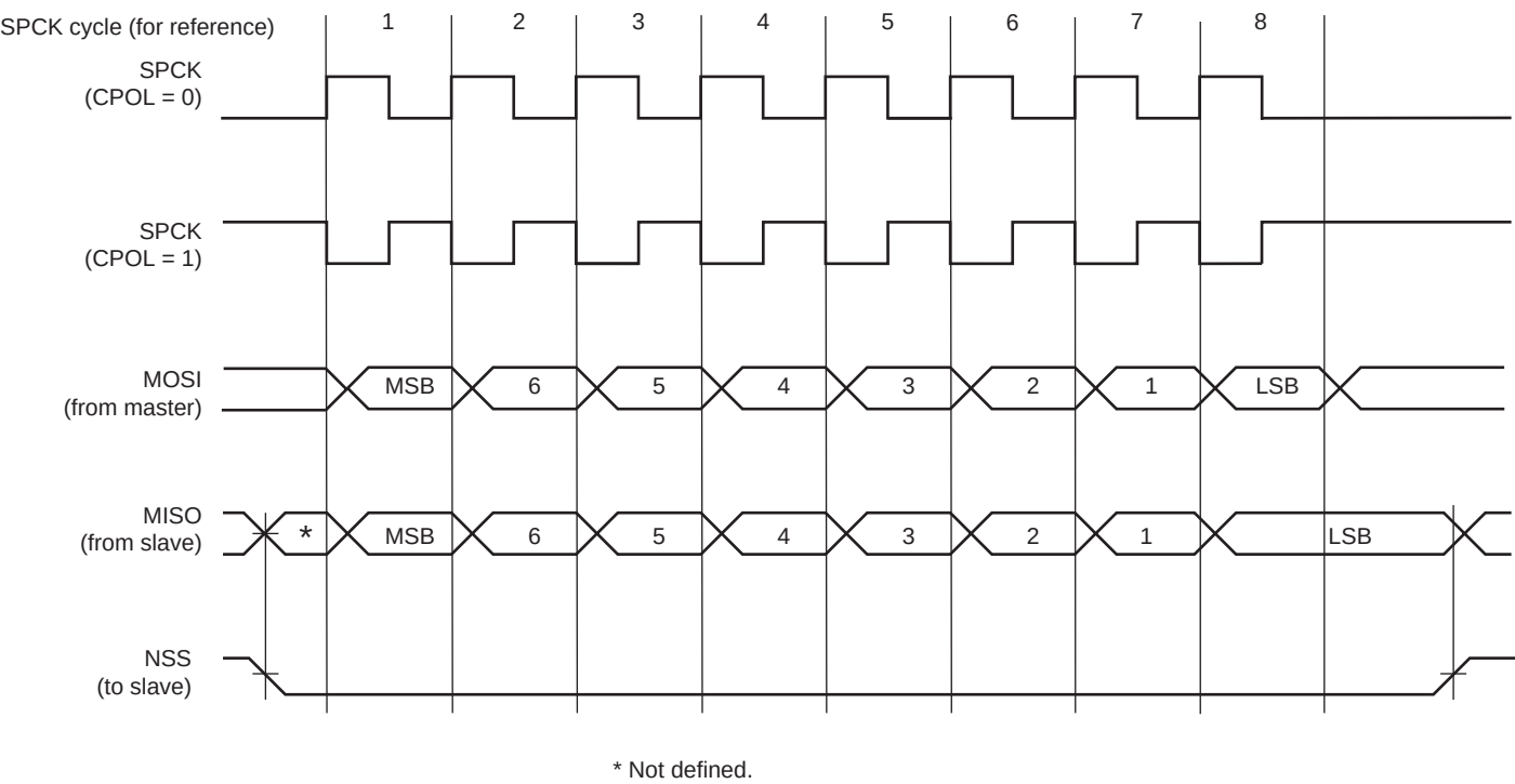
Figure 46-4. SPI Transfer Format (NCPHA = 0, 8 bits per transfer)
