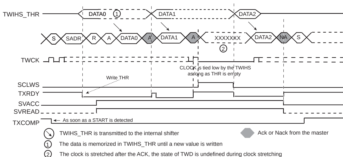
Figure 43-39. Clock Stretching in Read Mode
