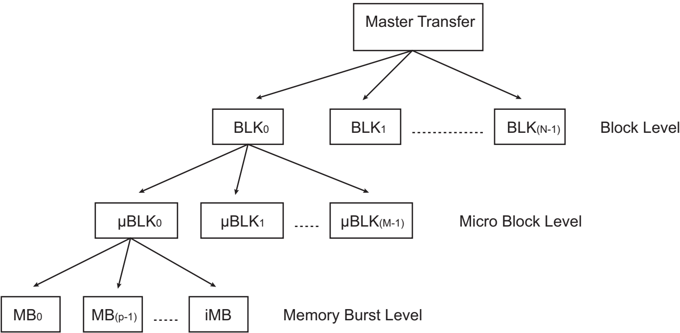
Figure 35-2. XDMAC Memory Transfer Hierarchy
