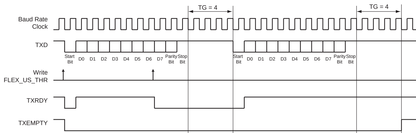
Figure 44-22. Timeguard Operations
