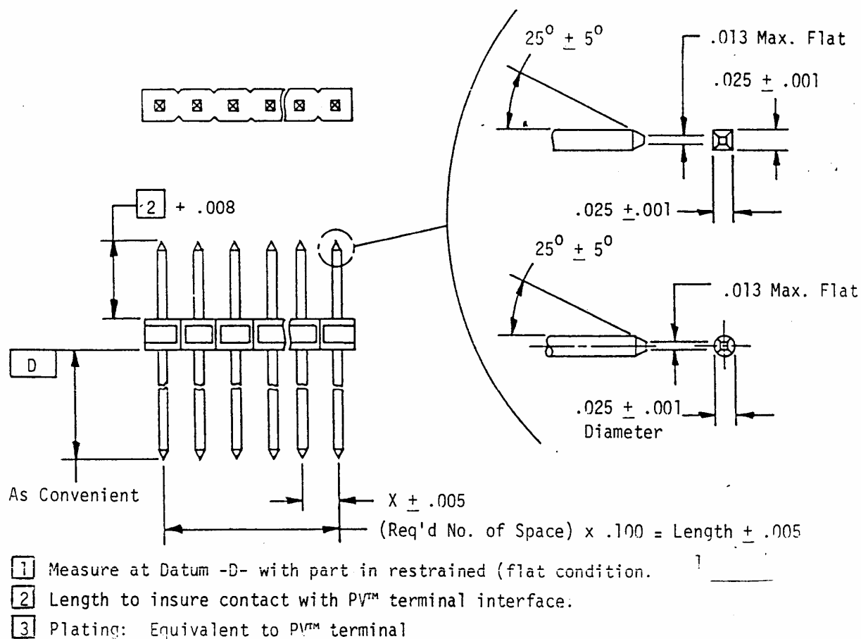
FIGURE 6 - MATING HEADER
