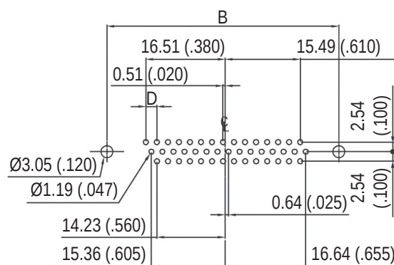
44 PIN
