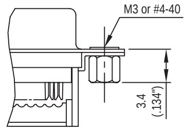
Threaded rear insert B / D
