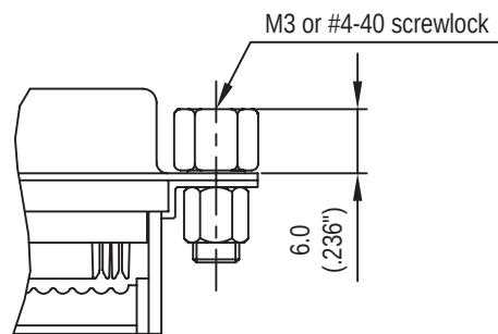
Front female screwlock A / C
