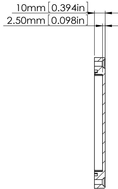
SECTION C-C
