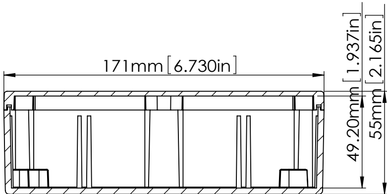
ASSEMBLY
