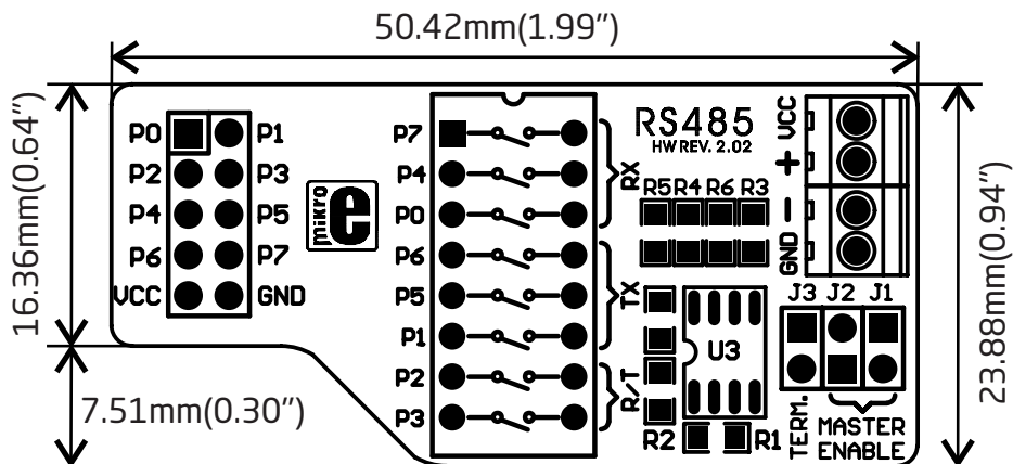
Figure 6-1: Dimensions
