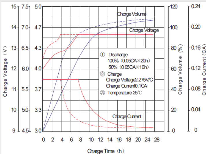
Charge characteristics
