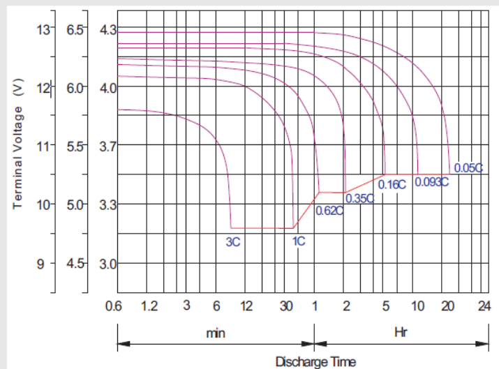
Discharge characteristics
