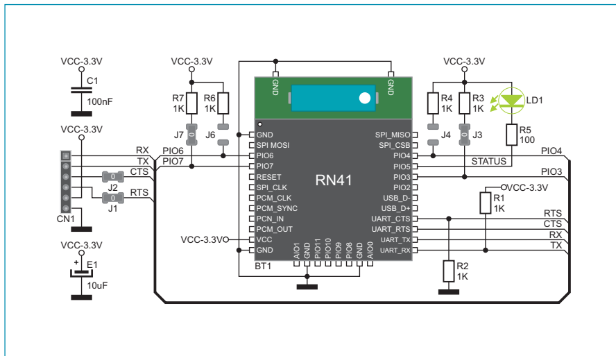
Figure 2: BlueTooth Stick connection shematic
