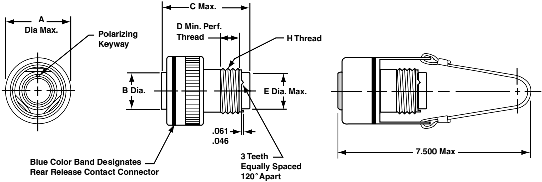
9818 CONNECTOR
