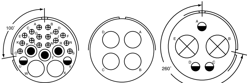
100° Rotation of 32-6
