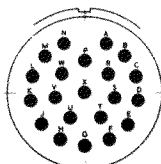
22-21 21 NO.16 CONTACTS
