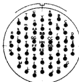
22-55 55 NO.20 CONTACTS
