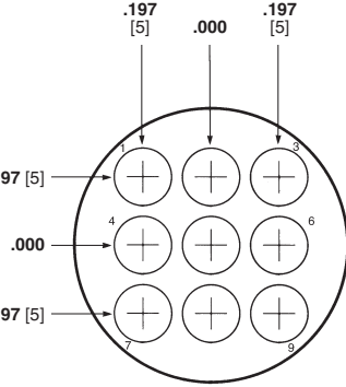
Arrangement 17-9 Max. Wire Ins. Dia. = .150 [3.81]
