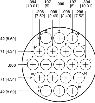
Arrangement 23-19 Max. Wire Ins. Dia. = .150 [3.81]
