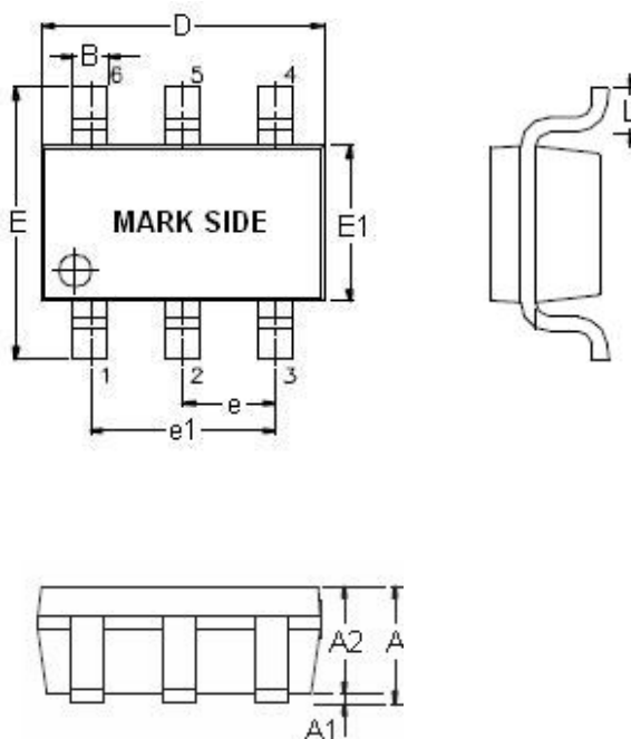
SOT-23- 6 Package (Unit: mm)
