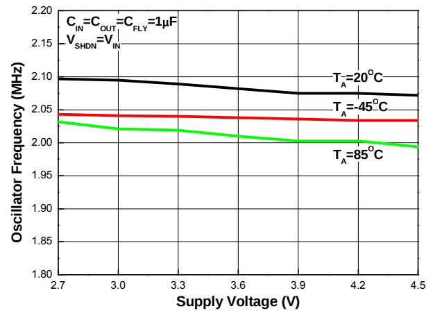
Figure 7. Oscillator Frequency vs. Supply Voltage
