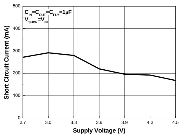
Figure 9. Short Circuit Current vs. Supply Voltage
