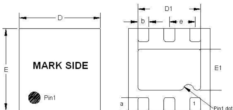
TDFN- 6 1.6mmX1.6mm Package (Unit: mm)
