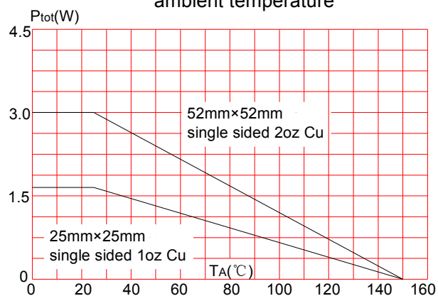
FIG.6 Total power dissipation versus ambient temperature
