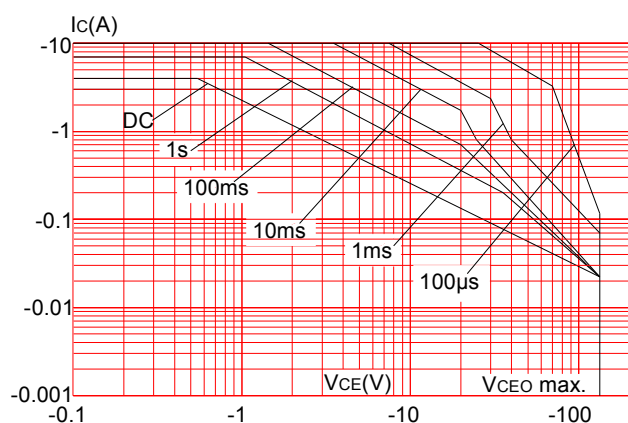
FIG.5: Area of safe operation
