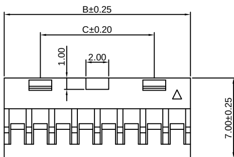
2x7P~2x25P A2005HB-N-2xXP-D
