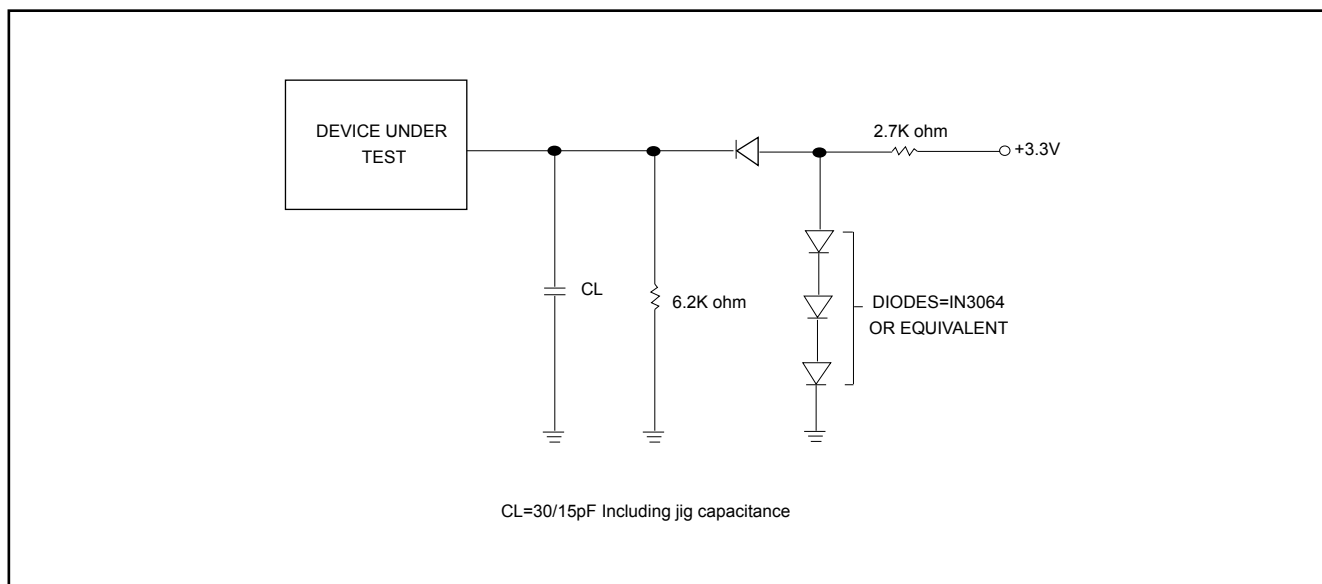
Figure 50. Output Loading
