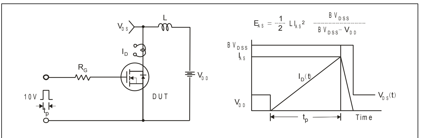
Fig.13 Unclamped Inductive Switching Test Circuit &amp; Waveform
