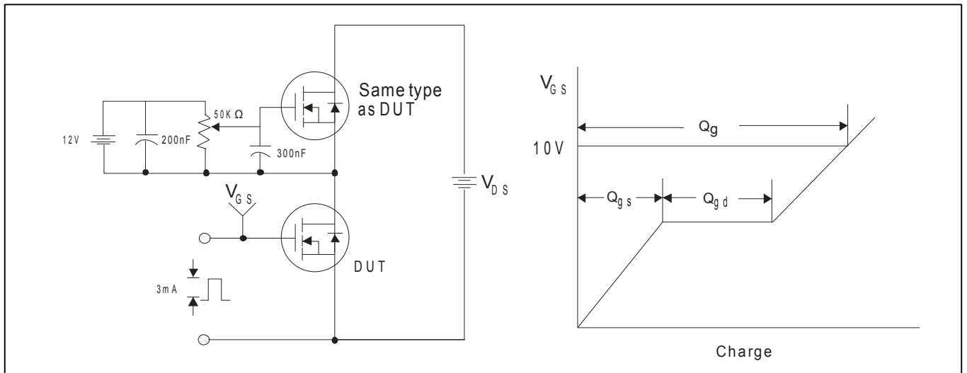
Fig.11 Gate Test circuit &amp; Waveform
