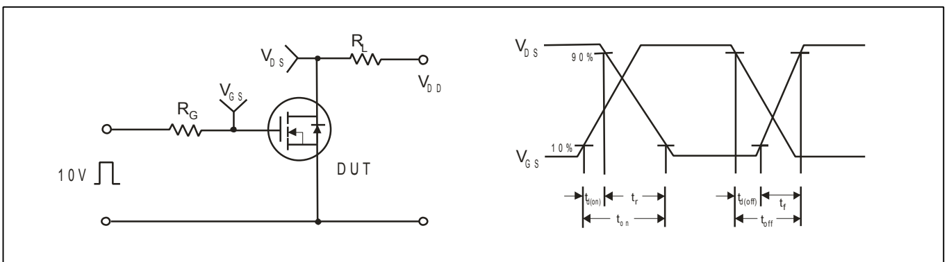
Fig.12 Resistive Switching Test Circuit &amp; Waveform
