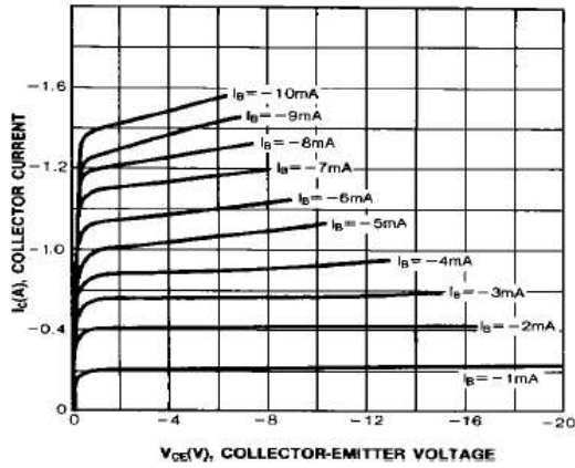
STATIC CHARACTERISTIC
