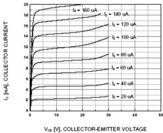
Figure 1. Static Characteristic
