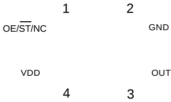
Pin Assignments
