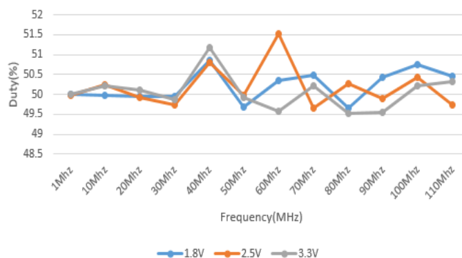
Figure 4. Duty Cycle vs Frequency
