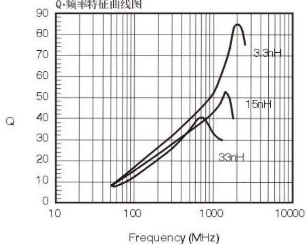
Q vs FREQUENCY CHARACTERISTICS Q·频率特征曲线图
