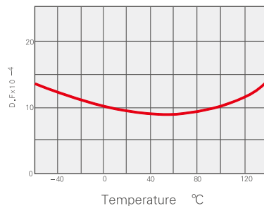
CG 损耗角正切曲线 D.F.vs Temperature
