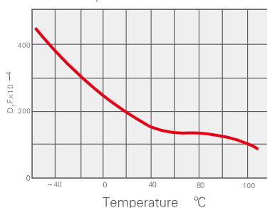
2X1 损耗角正切曲线 D.F.vs Temperature
