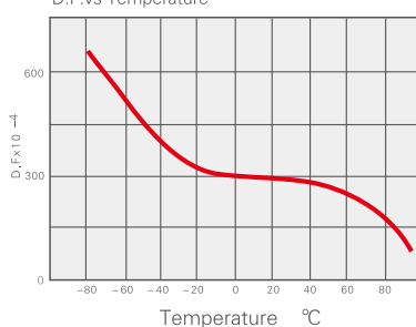
X5R 损耗角正切曲线 D.F.vs Temperature
