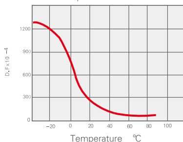
2F4 损耗角正切曲线 D.F.vs Temperature
