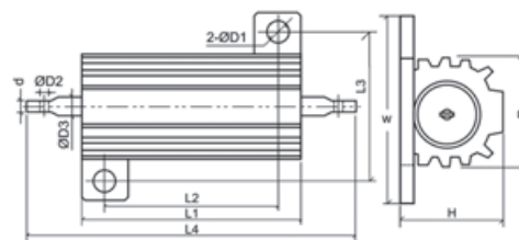
PDM5W~50W
