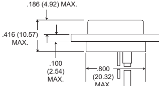
Plug
