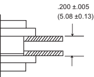
Plug and Receptacle Rear Mounted
