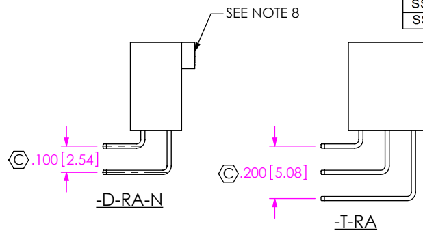
FIG 2 RIGHT ANGLE OPTION ALL OPTIONS DIFFERENT AS SHOWN, OTHERWISE SAME AS -S-RA
