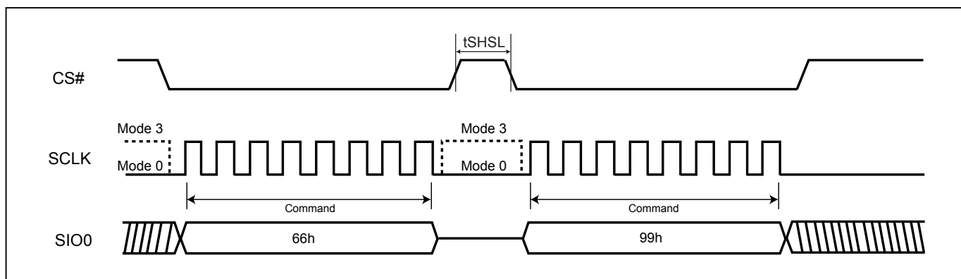
Figure 36. Reset Sequence
