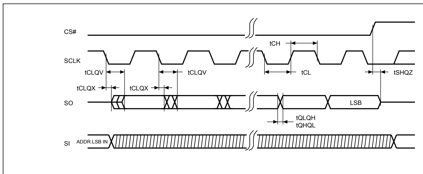
Figure 33. Output Timing
