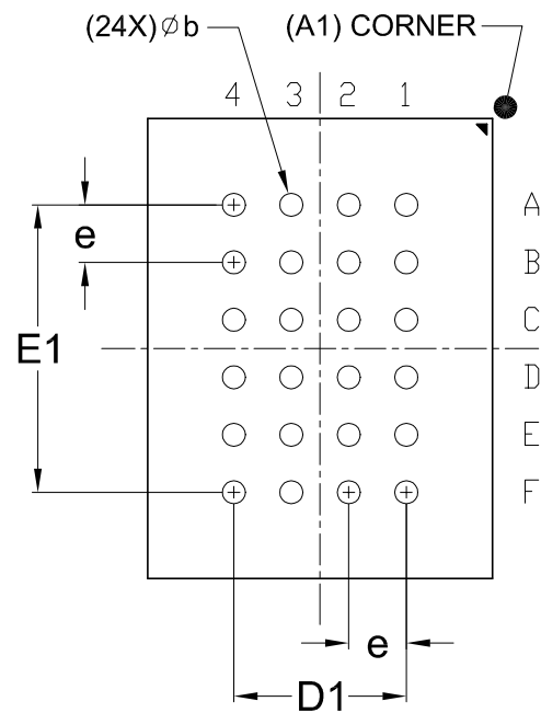
BOTTOM VIEW
