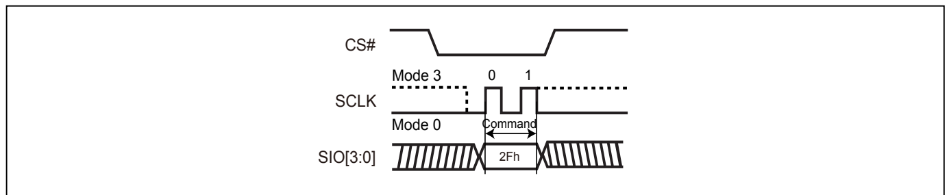
Figure 69. Write Security Register (WRSCUR) Sequence (QPI Mode)
