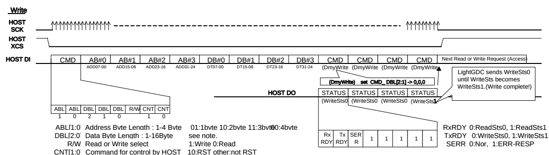
Figure 4-2 Write access
