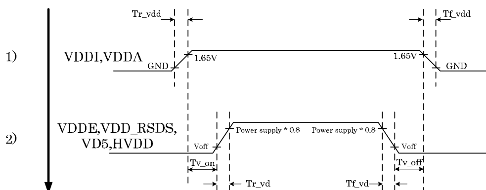
Power ON Sequence
