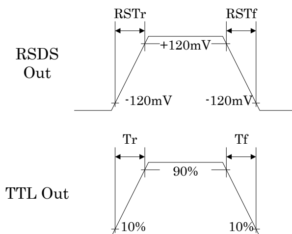
Figure 32-10 Rise Fall Times
