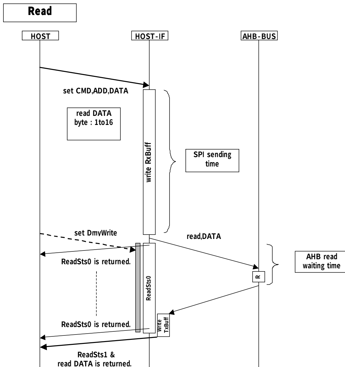
Figure 4-5 Read process flow
