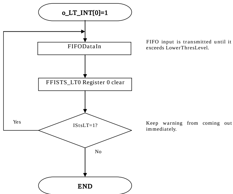
Figure 22-11 FIFO Lower Threshold Warning Flow
