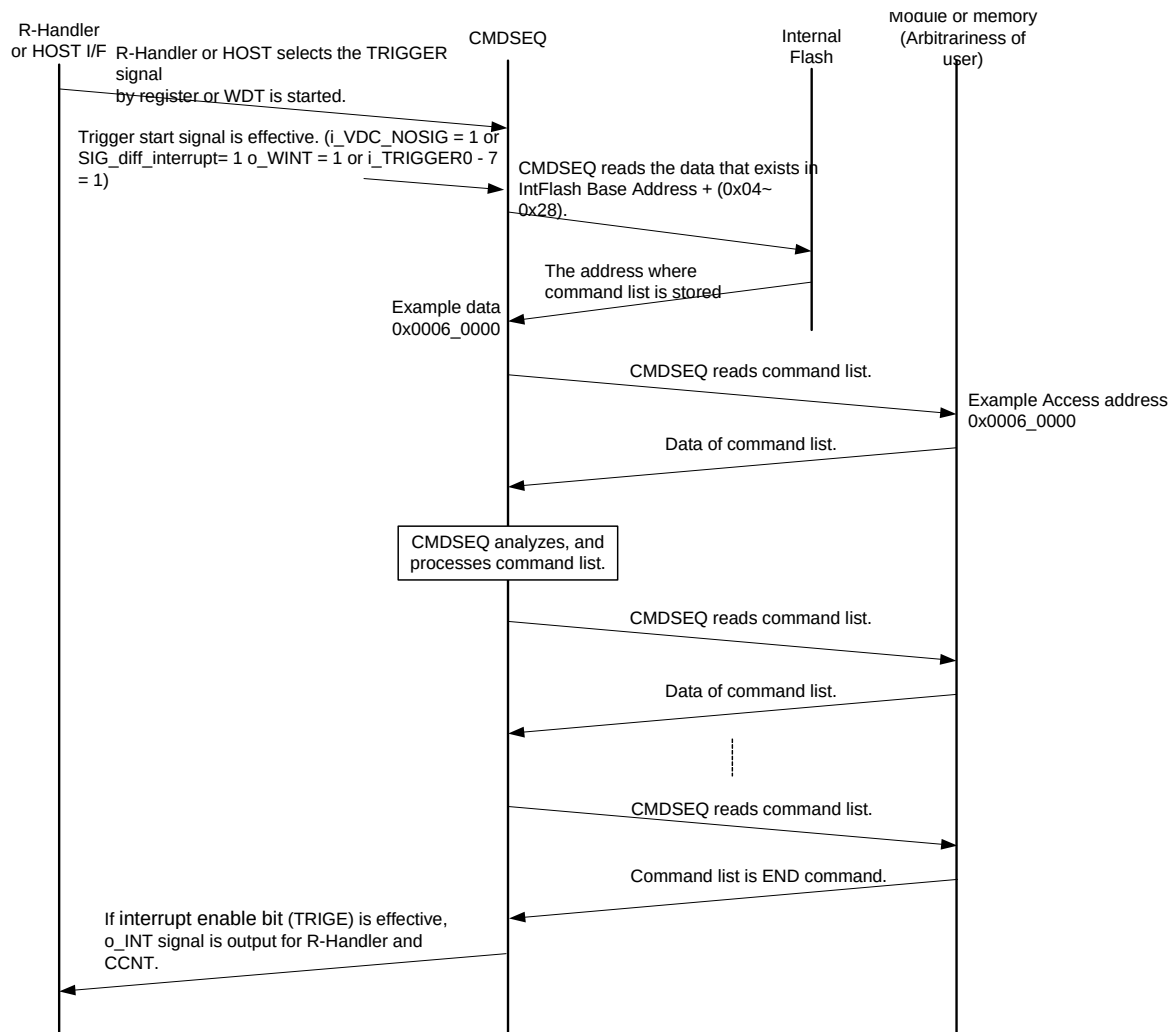
Figure 7.3-4 Trigger start
