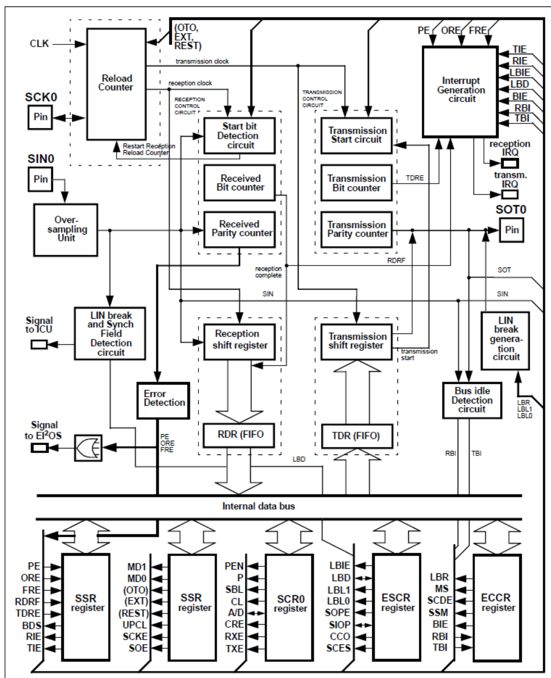
Figure 26-1 Block Diagram
