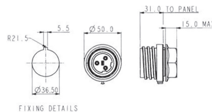
FIXING DETAILS
