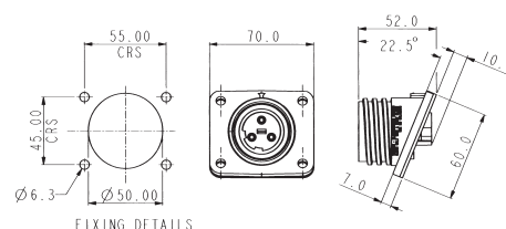
FIXING DETAILS
