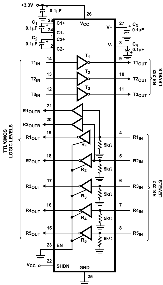
ICL3241
