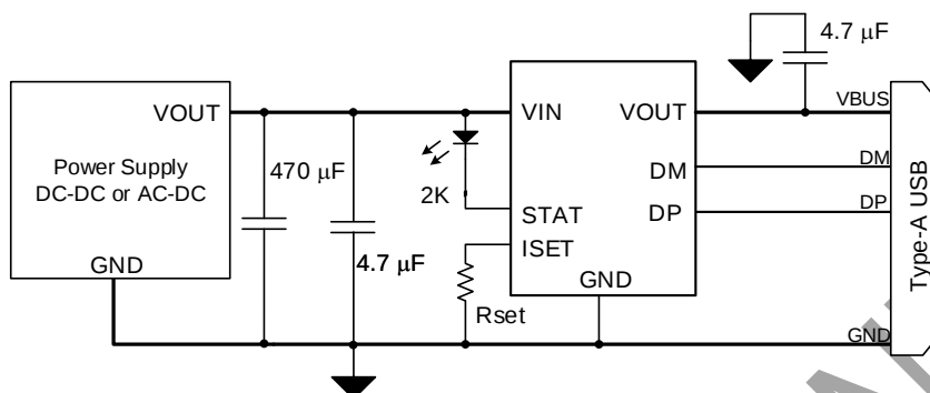
Figure 1 SC7004 typical application circuit
