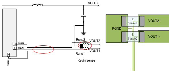
Figure.8 Current sense
