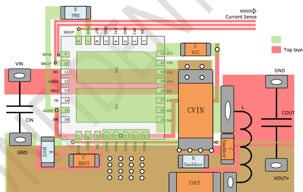
Figure.7 A layout example of SC8103
