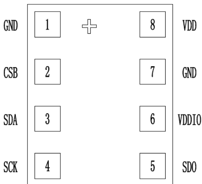
Figure 3: Layout pin configuration SPL06-007 (bottom view)
