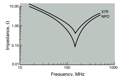
Variation of Impedance with Ceramic Form Impedance vs. Frequency 1000 pF - C0G (NP0) vs. X7R 0805
